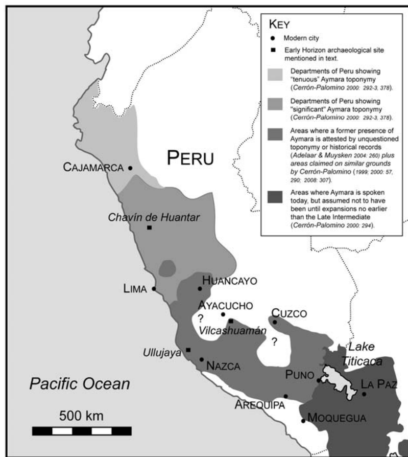
Figure 3: Current and assumed earlier distributions of Aymara, by nature and strength of evidence
